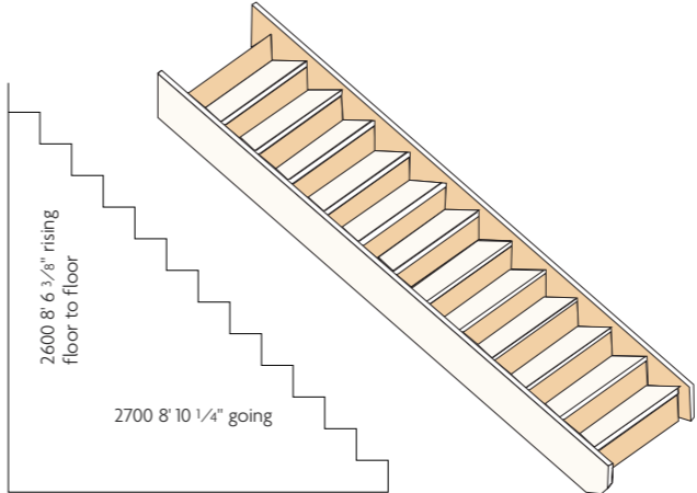
12 TREAD 13 RISERS*
